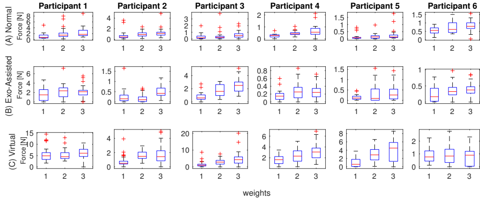
Fig. 4. The box plots show the magnitude of the grip force overshoot during the initial phase of the lift-off for all six participants and conditions. The overshoot is quantified as the force difference between the peak of force after the lift-off and the lowest point of the force pattern in the range of 1s after the peak. A correlation between the overshoot magnitude and the weight is observed for the majority of participants.
