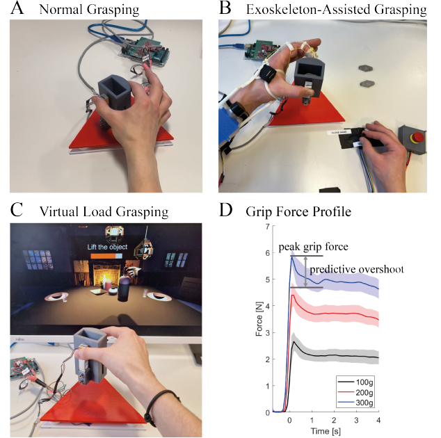
Fig. 1. Grasp force dynamics experiments in different neurorehabilitation settings: A) Participants grasp and lift an object with three different load weights while their pinch grip force is measured with a load cell attached to the object B) Participants control a tendon-driven soft hand exoskeleton to assist them during pinch grasping. The turn knob can be used to flex/extend the finger. C) Participants grasp and lift objects in a virtual environment. They can only lift the virtual object (bottle) if they apply more than the object-specific threshold force on the physical grasp interface D) The characteristic grip force profiles when healthy individuals grasp and lift objects of different weights.
