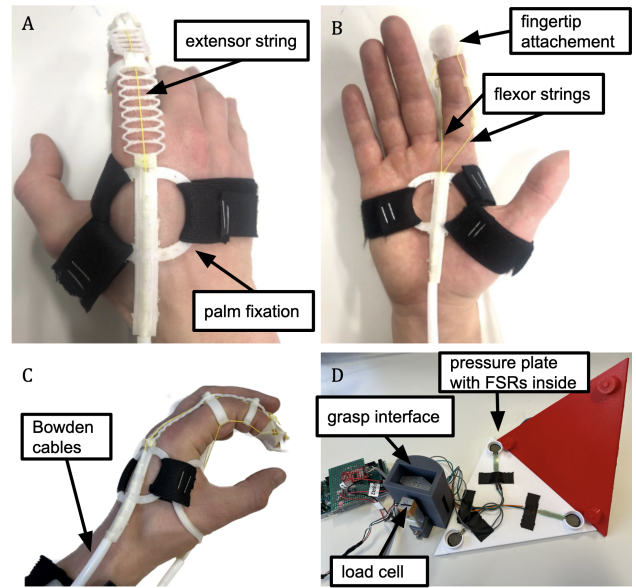
Fig. 2. Tendon-driven and light-weight soft exoskeleton composed from modular 3D-printed parts. A) Dorsal view on the hand exoskeleton with visible extensor tendons B) Palmar view on the hand exoskeleton with visible flexor tendons C) Side view on the hand exoskeleton during pinch grip. The tendons are routed inside Bowden cables towards the spool of the DC motor D) The adjustable weight box with the attached load cell is used as grasp interface for our grip force measurements. To detect the exact time points when the object is lifted and placed down, we use a triangular pressure plate with three force sensitive resistors underneath. All sensors are connected to a microcontroller where there data is processed and recorded.
